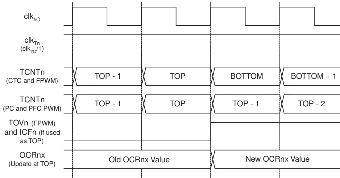
Figure 12-14. Timer/Counter Timing Diagram, no Prescaling
