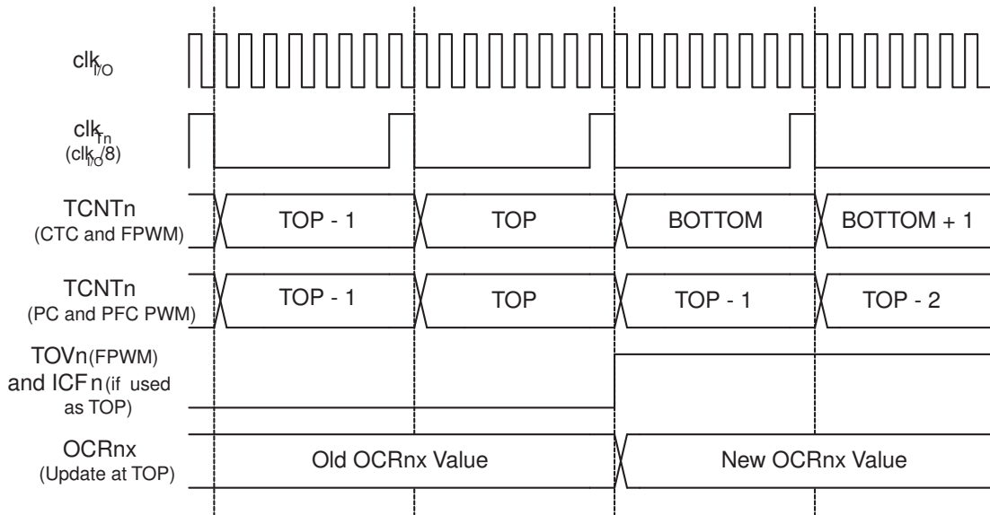
Figure 12-15. Timer/Counter Timing Diagram, with Prescaler ( f_{clk\_I/O}/8 )
