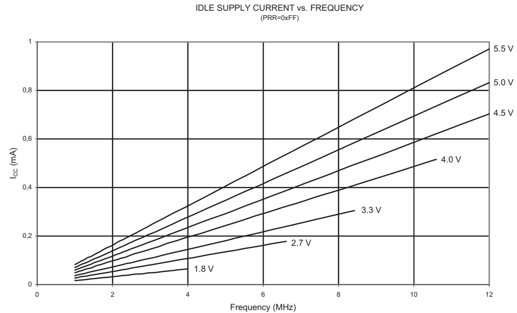
Figure 18-8. Idle Supply Current vs. Frequency (1 - 12 MHz)
