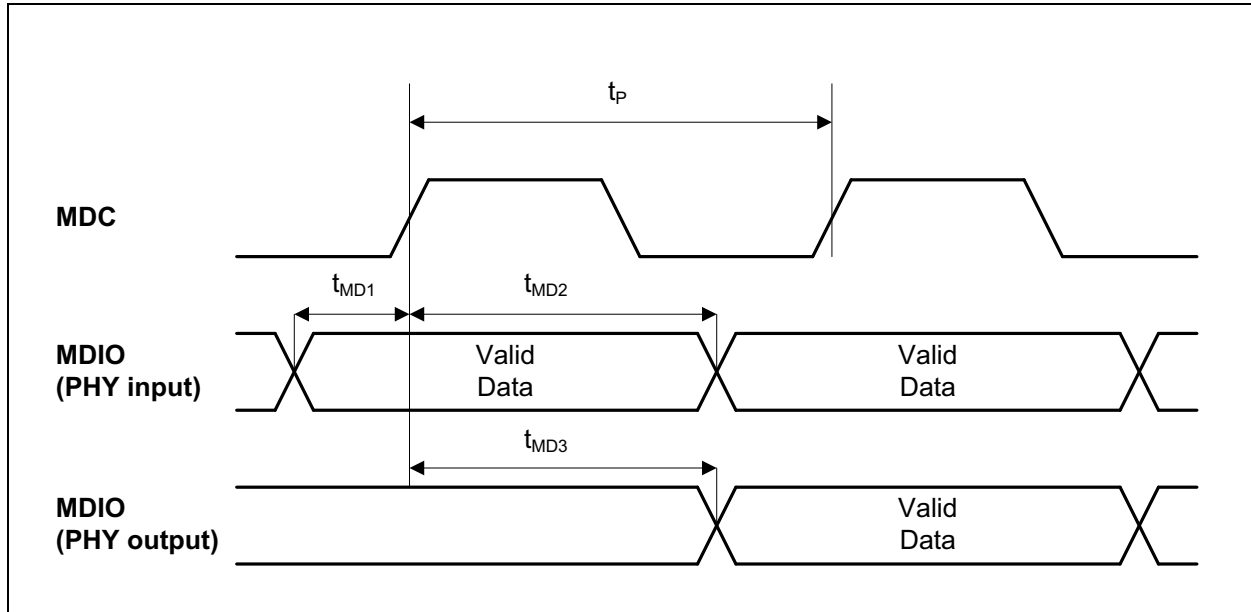
FIGURE 7-11: MDC/MDIO TIMING
