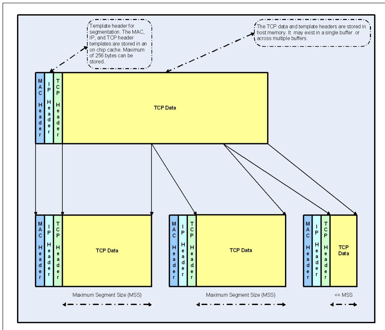
FIGURE 6-4: TCP SEGMENTATION
