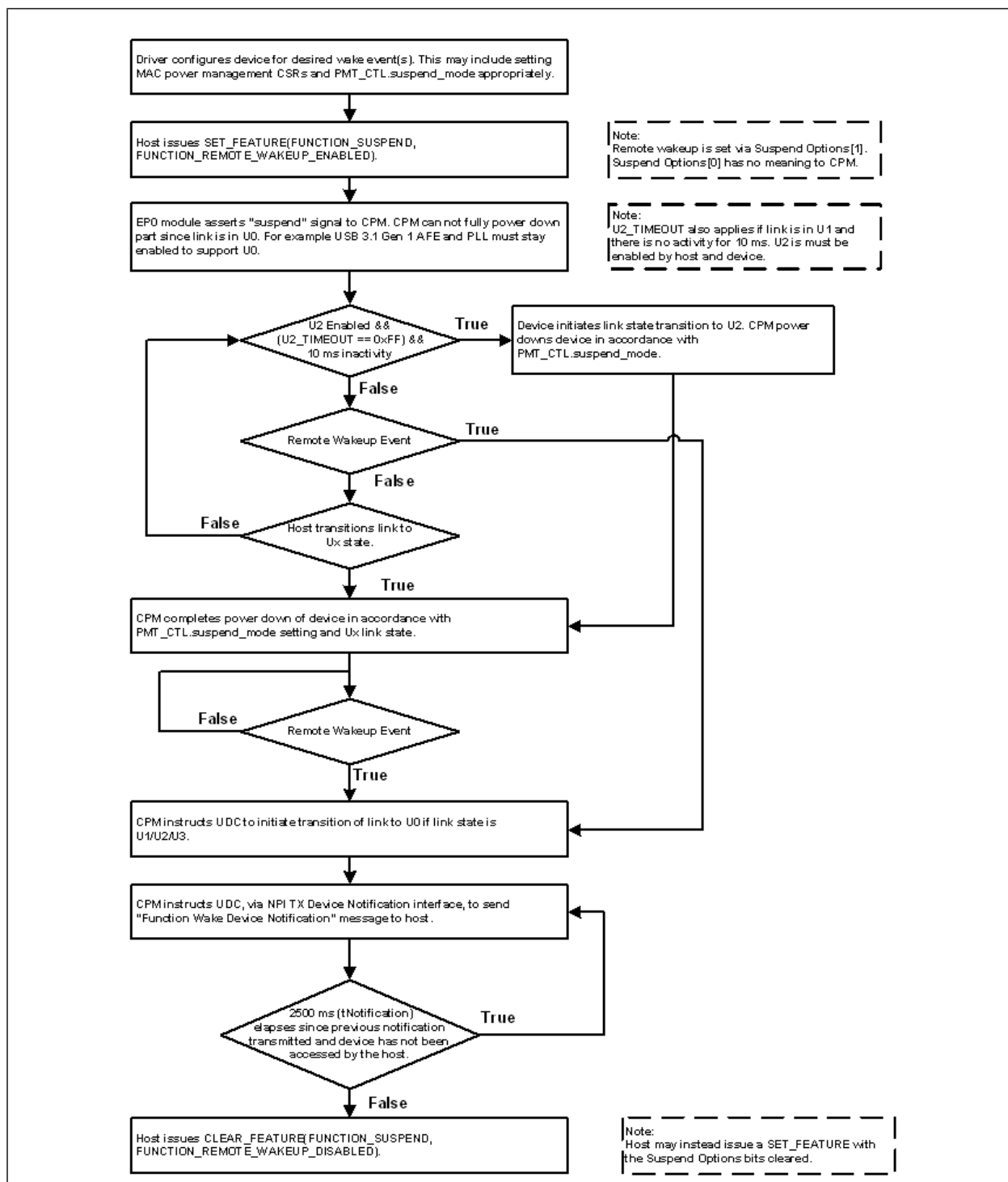
FIGURE 5-2: FUNCTION SUSPEND
