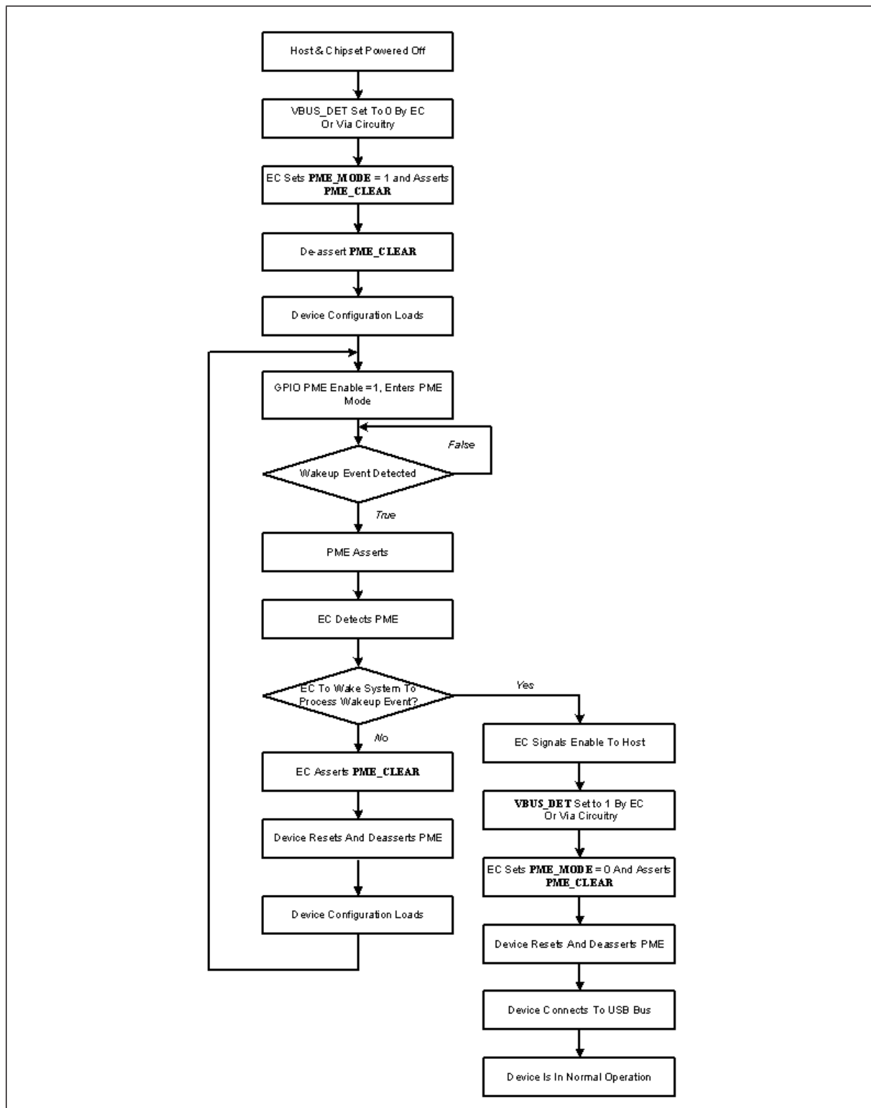
FIGURE 14-2: PME OPERATION
