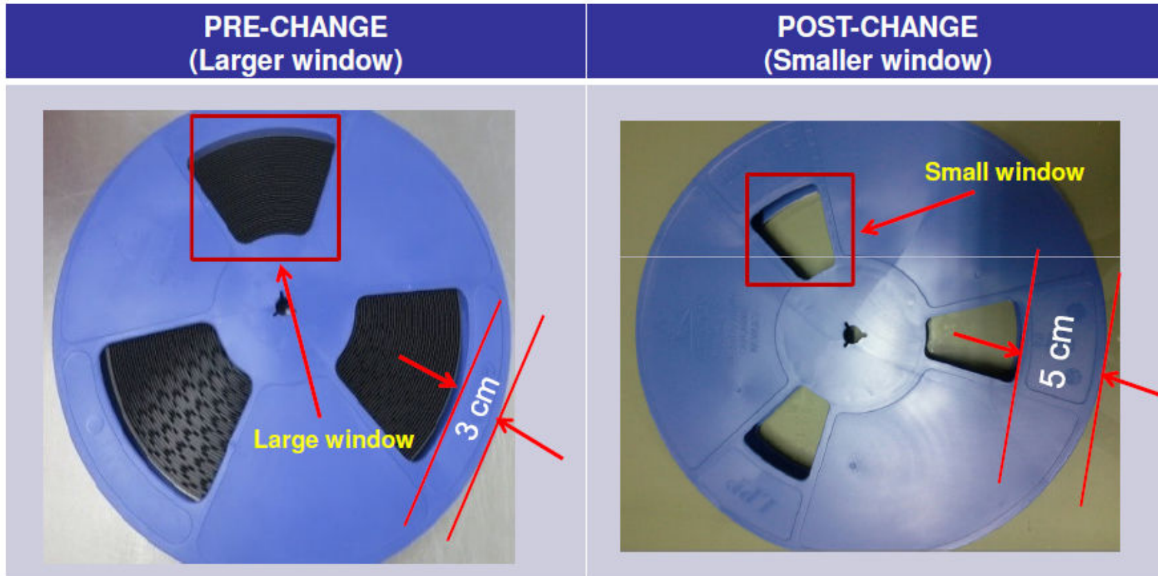
Fig 1. Current and new design of plastic reel
