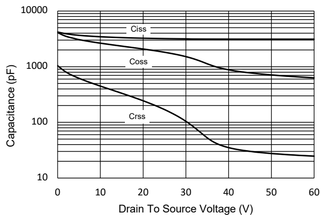
Fig.5 - Capacitance Characteristics
