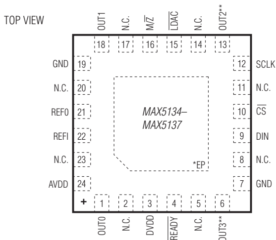
THIN QFN (4mm x 4mm)
