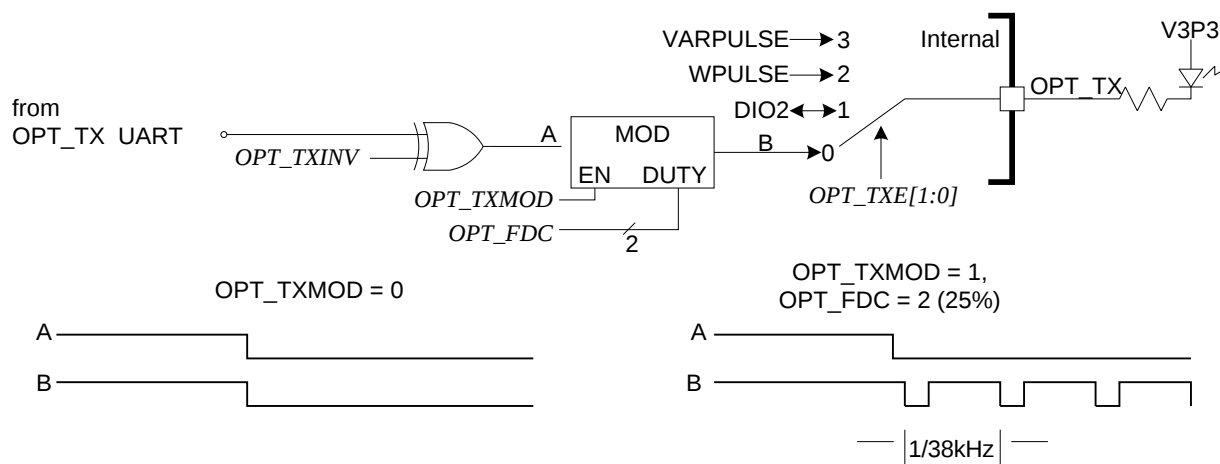
Figure 14: Optical Interface
