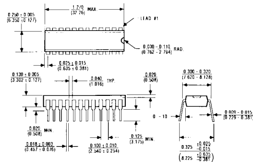
24 Lead Plastic Narrow DIP (NG)
