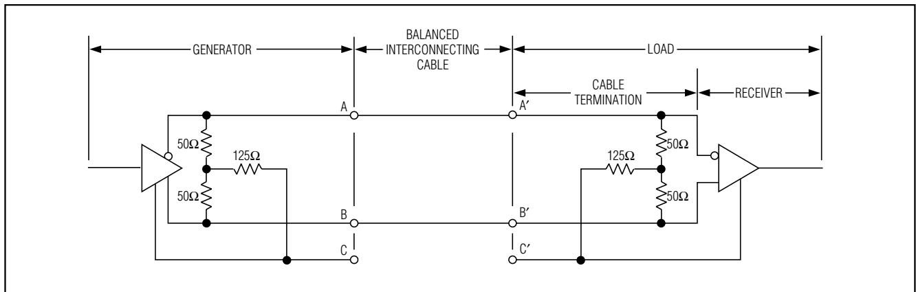
Figure 11. Typical V.35 Interface
