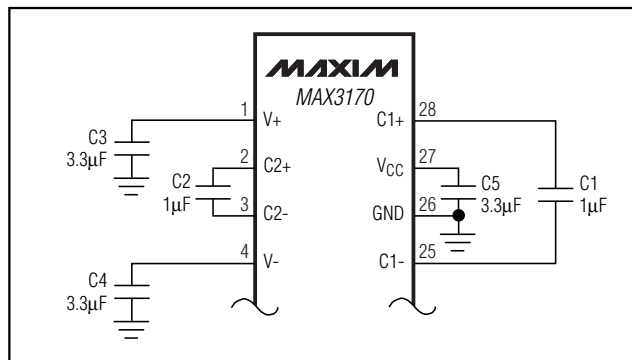
Figure 6. Charge-Pump Connections
