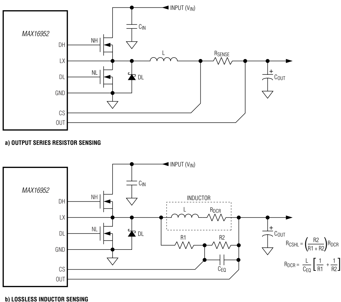
Figure 4. Current-Sense Configurations
