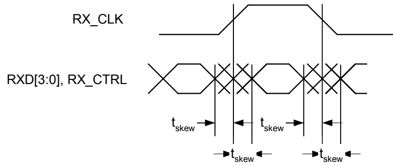
Figure 17: RGMII RX_CLK Delay Timing - Register 28.11:10 = 00
