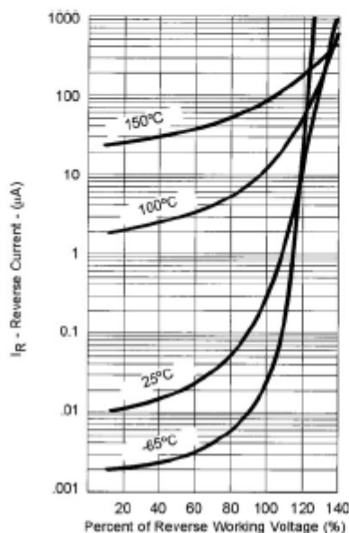
FIGURE 4 Typical Reverse Current vs Reverse Voltage
