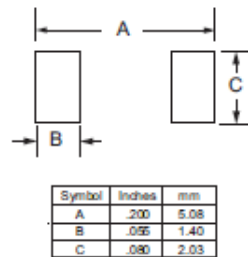
PAD LAYOUT
