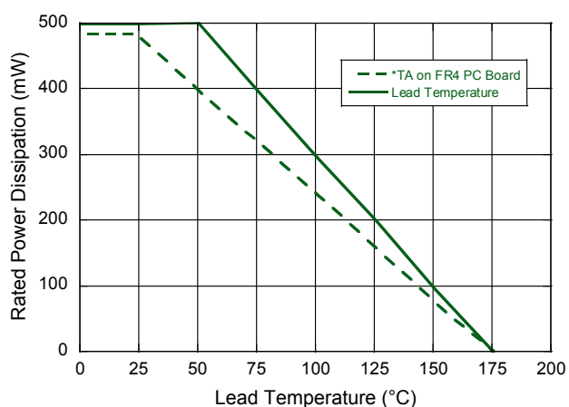
Power Derating vs. Lead Temperature
