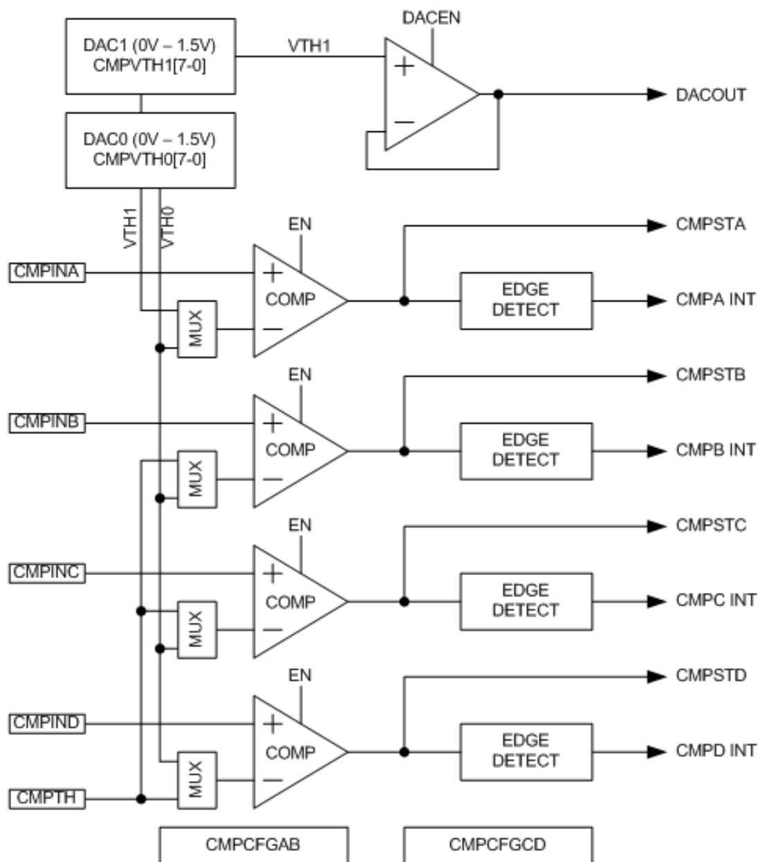
CMPCFGAB (0xA038h) Analog Comparator A/B Configuration Register R/W (0x00)
