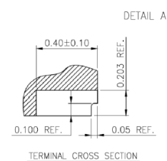
TERMINAL CROSS SECTION
