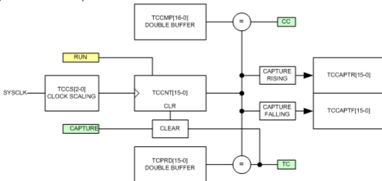
TCCFG1 (0xA050h) TCC Configuration Register 1 R/W (0x00)
