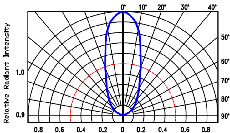
Fig.5 Radiation Diagram
