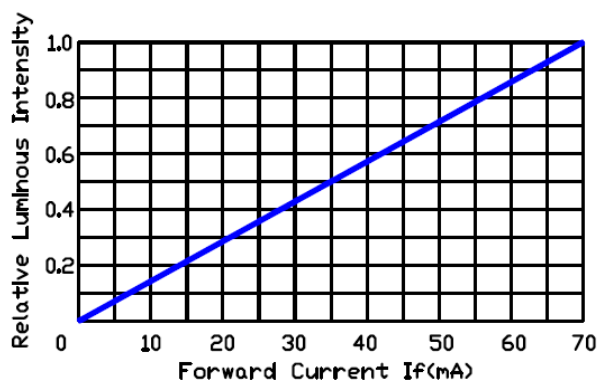
Fig.4 Relative Intensity vs Forward Current
