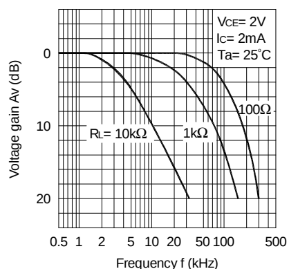
Fig.11 Frequency Response
