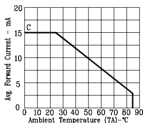
Fig5. MAX. AVERAGE FORWARD CURRENT VS. AMBIENT TEMPERATURE
