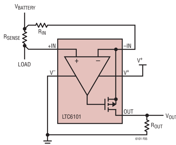
Figure 5. V + Powered Separately from Load Supply (V BATT )
