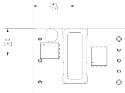
Figure 15. Pick and Place Location.
