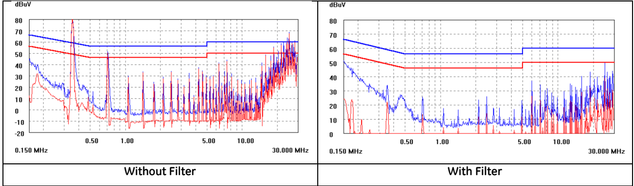
Figure 20. EMC Considerations
