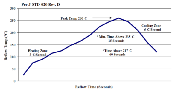
Figure 18. Recommended linear reflow profile using Sn/Ag/Cu solder.
