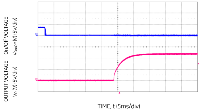
Figure 5. Typical Start-up Using Remote On/Off, negative logic version shown ( V_{IN} = 48V, I_o = I_{o,max} ).
