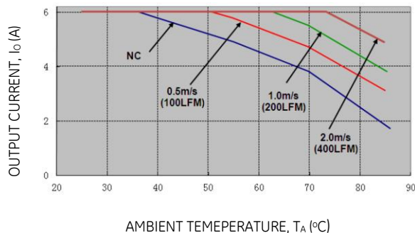
Figure 14. Output Current Derating for the Open Frame Module; Airflow in the Transverse Direction from V_{out}(+) to V_{out}(-) ; V_{in} = 48V .
