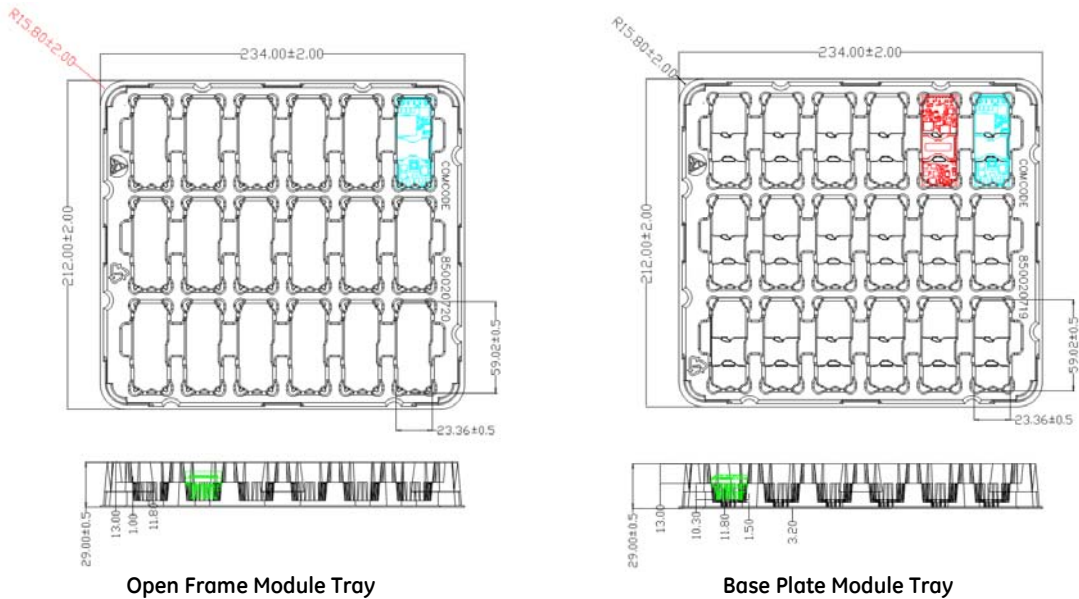
Open Frame Module Tray Figure 25. EBVW025 Packaging Tray
