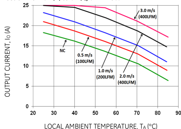
Figure 21. Output Current Derating for the Base plate EBDW025A0B-H in the Transverse Orientation; Airflow Direction from V_{in}(+) to V_{in}(-) ; V_{in} = 48\text{ V} .
