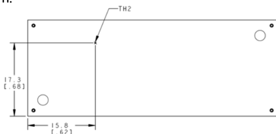
Figure 19. Location of the thermal reference temperature TH_2 for Baseplate module.
