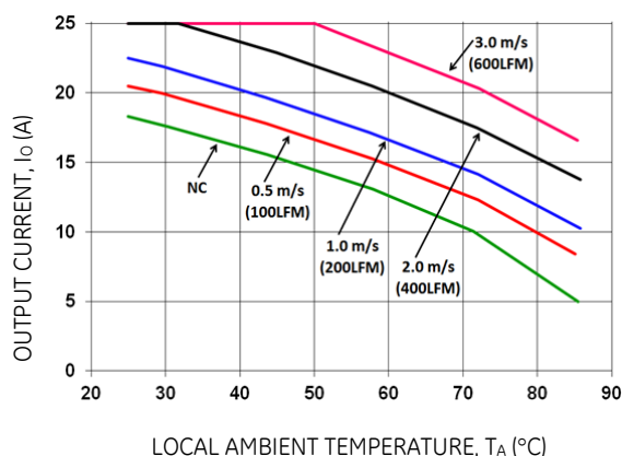
Figure 20. Output Current Derating for the Open Frame EBDW025A0B in the Transverse Orientation; Airflow Direction from V_{in}(+) to V_{in}(-) ; V_{in} = 48\text{ V} .
