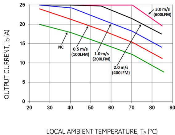
Figure 22. Output Current Derating for the Base Plate EBW025A0Bxx-H and 0.25" heat sink in the Transverse Orientation; Airflow Direction from Vin(-) to Vin(+); Vin = 48V.
