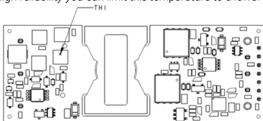
Figure 18. Location of the thermal reference temperature TH_1 .
