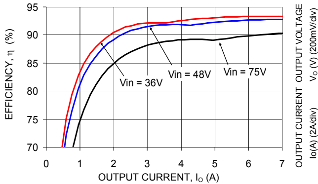
Figure 1. Converter Efficiency versus Output Current.
