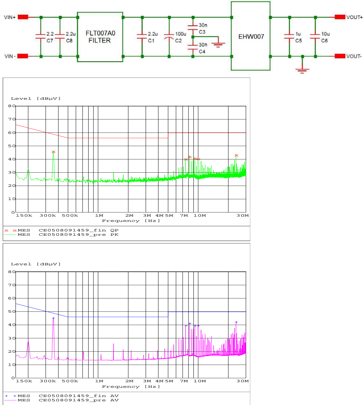
Figure 21. EMC Considerations
