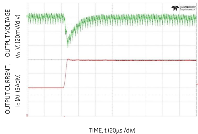
Figure 16. Transient Response to Dynamic Load Change from 50% to 100% at 12V in , C_{out} = 7\text{X}47\mu\text{F} + 2\text{X}330\mu\text{F} , C_{Tune}=3900\text{pF} , R_{Tune}=300
