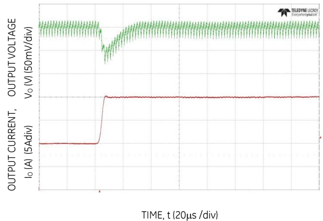
Figure 28 Transient Response to Dynamic Load Change from 50% to 100% at 12V in , C_{out} = 4 \times 47\mu\text{F} + 1 \times 330\mu\text{F} , C_{Tune}=1800\text{pF} , R_{Tune}=300
