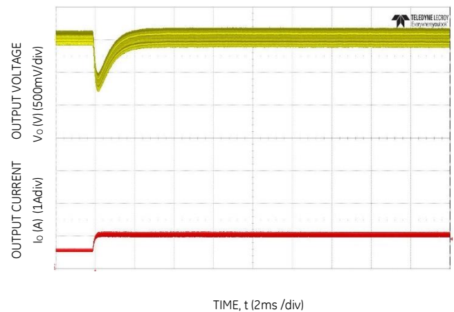
Figure 16. Transient Response to Dynamic Load Change from 0.65A to 1.15A at 12Vin, C_{out}=9\times 4.7\mu\text{F} , C_{Tune}=220\text{pF} , R_{Tune}=40.2\text{k}\Omega
