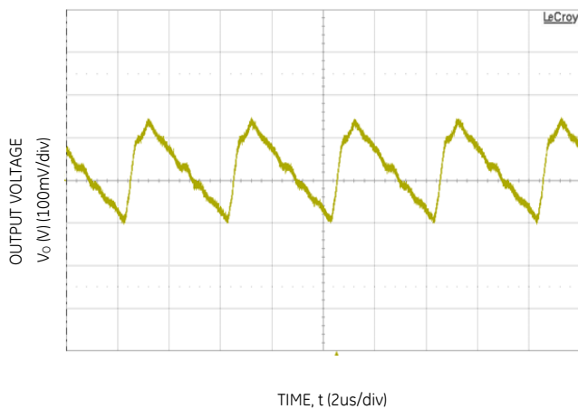
Figure 15. Typical output ripple and noise ( C_o=66\mu\text{F} ceramic, V_{IN} = 12\text{V} , I_o = I_{o,max} ).
