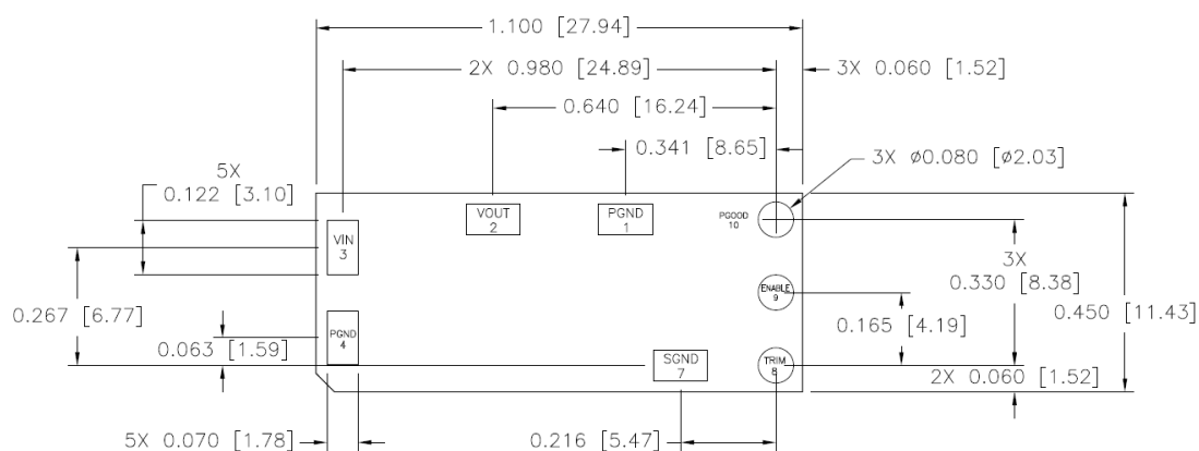
MODULE'S PWB FOOTPRINT LAYOUT (BOTTOM VIEW)
