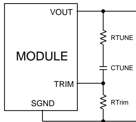
Figure 32. Circuit diagram showing connection of R_{\text{TUNE}} and C_{\text{TUNE}} to tune the control loop of the module
