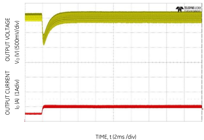
Figure 22. Transient Response to Dynamic Load Change from 0.6 to 1.1A at 12Vin, C out =7x4.7μF, C Tune =82pF, R Tune =40.2kΩ
