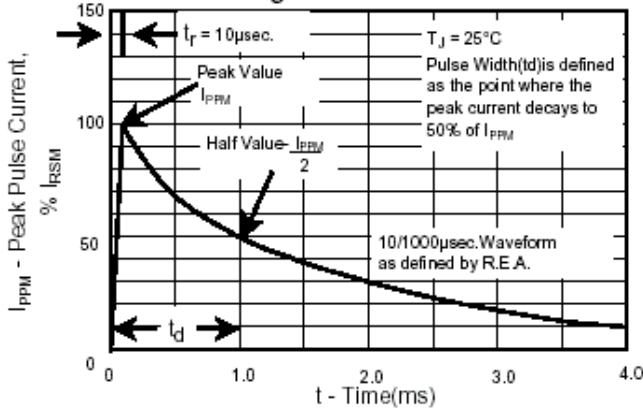
Fig.3 - Pulse Waveform
