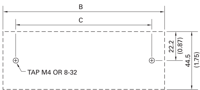
MOUNTING DETAIL
