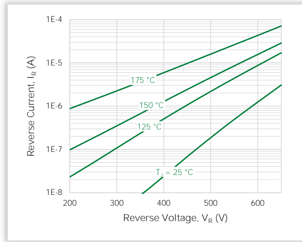
Figure 2. Typical Reverse Characteristics (Per Leg)
