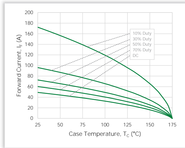
Figure 4. Current Derating (Per Leg)
