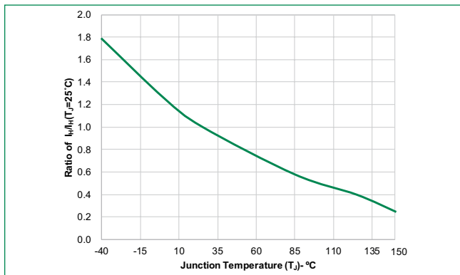
Figure 3: Normalized DC Holding Current vs. Junction Temperature
