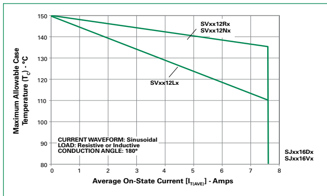
Figure 7: Maximum Allowable Case Temperature vs. Average On-State Current
