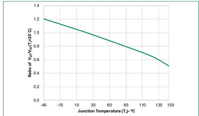
Figure 2: Normalized DC Gate Trigger Voltage vs. Junction Temperature
