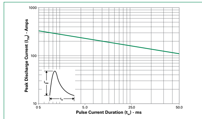
Figure 8: Peak Capacitor Discharge Current
