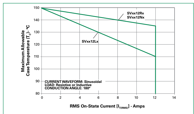
Figure 6: Maximum Allowable Case Temperature vs. RMS On-State Current
