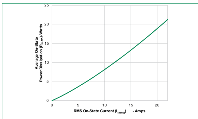
Figure 5: Power Dissipation (Typical) vs. RMS On-State Current
