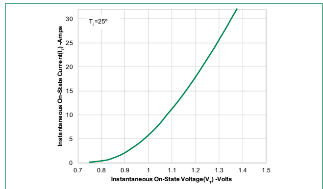
Figure 4: On-State Current vs. On-State Voltage (Typical)
