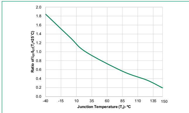
Figure 1: Normalized DC Gate Trigger Current vs. Junction Temperature
