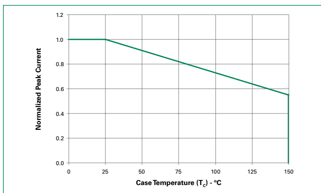
Figure 9: Peak Capacitor Discharge Current Derating
