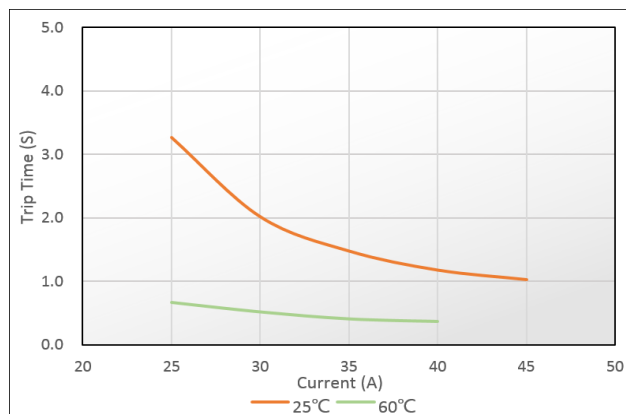
Open Time vs. Current Curves – @ 25°C & 60°C
