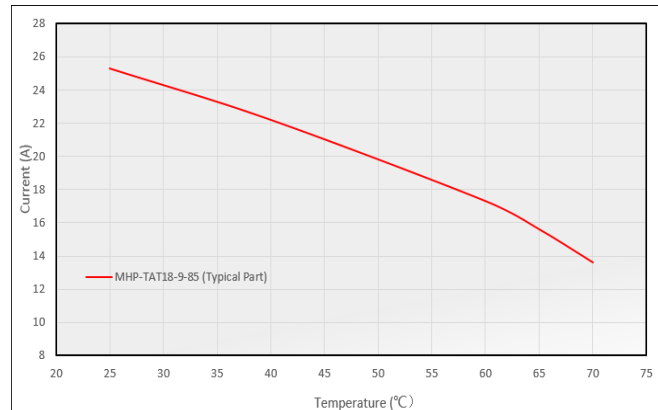
Current vs. Temperature Curve*
