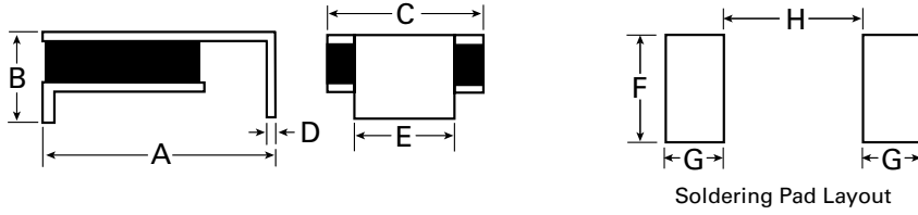
Soldering Pad Layout
