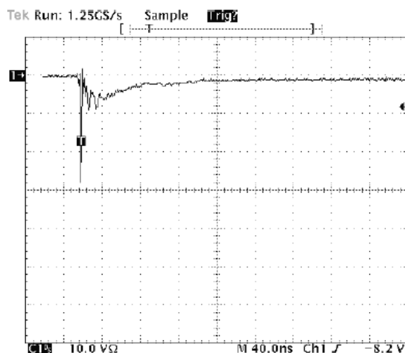
Fig 5. Negative 8kV contact per IEC 61000-4-2-LESD8D12T5G
