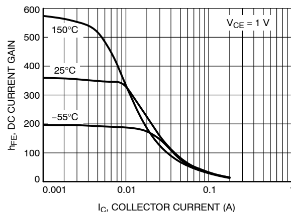
Figure 9. DC Current Gain vs. Collector Current
