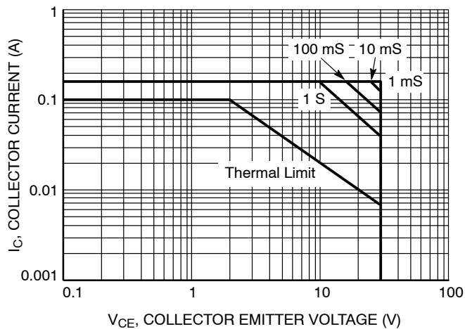
Figure 35. Safe Operating Area for LBC848A, LBC848B, LBC848C
