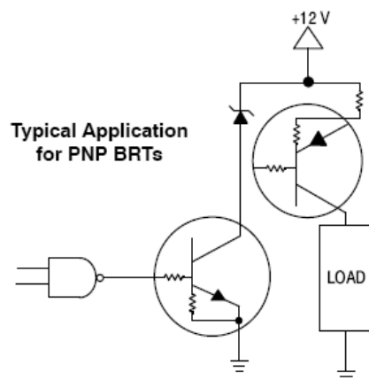
Figure 47. Inexpensive, Unregulated Current Source
