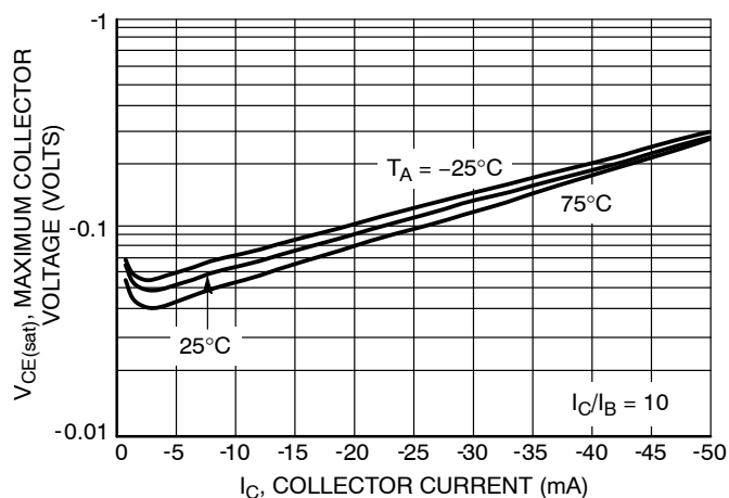
Figure 53. Maximum Collector Voltage vs. Collector Current
