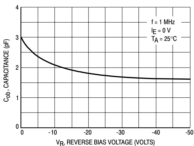
Figure 9. Output Capacitance
