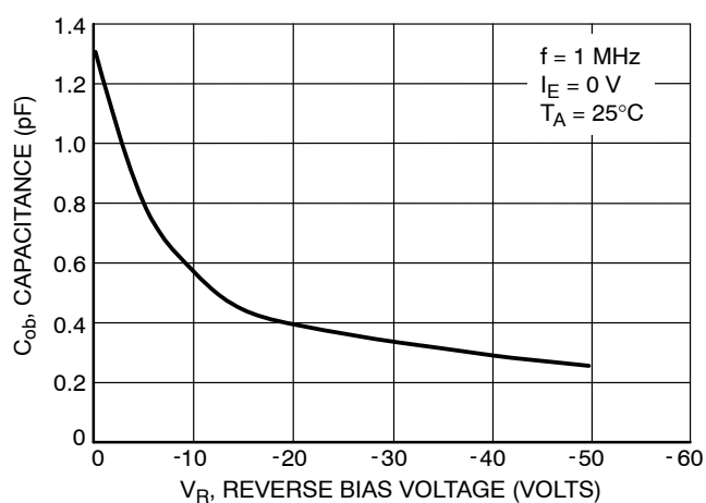
Figure 55. Output Capacitance
