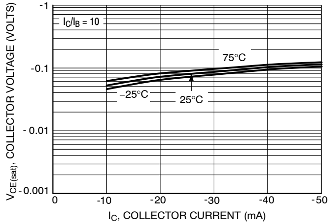
Figure 27. V_{CE(sat)} versus I_C
