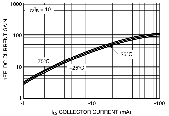
Figure 33. DC Current Gain
