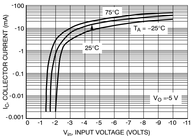
Figure 56. Output Current vs. Input Voltage
