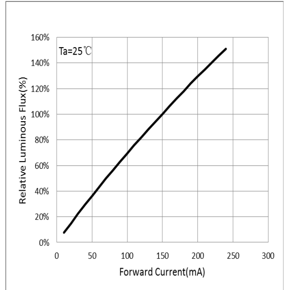
I_f ----- Relative Luminous flux
