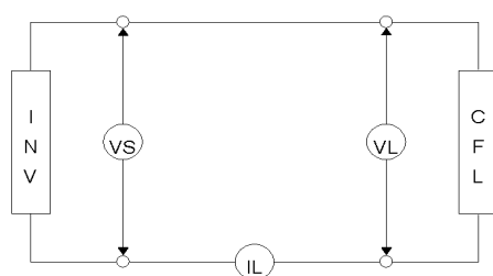
CFL Testing Circuit
