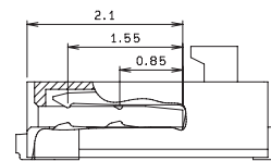
SECT. X-X
