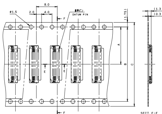
SECT. F-F
