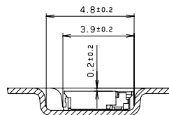
SECT. X-X
