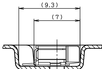
SECT. E-E (S=4:1)
