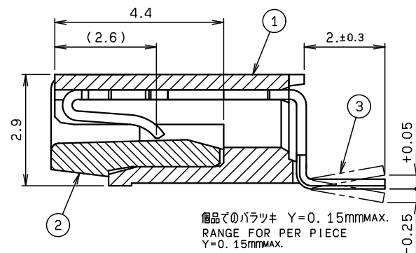
SECT. X-X (S=10:1)
