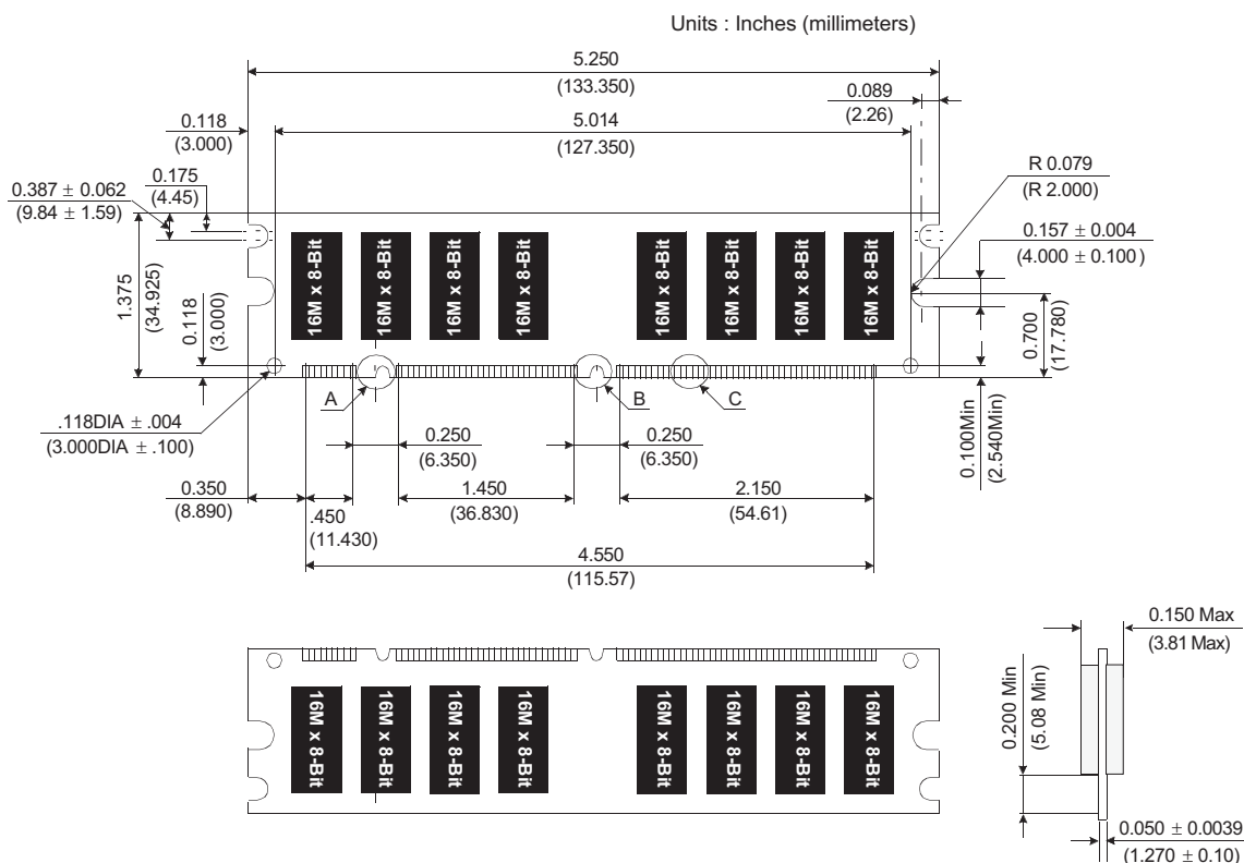
Figure 1: KVR100X64C3/256 168-Pin SDRAM Module
