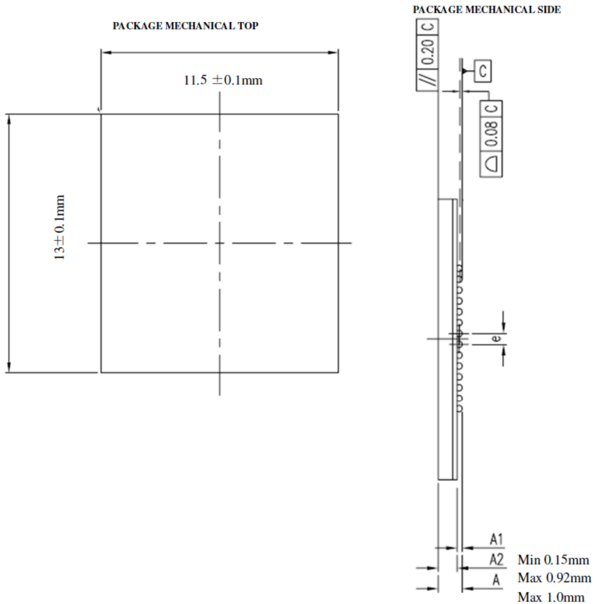
Figure 2 – Package Dimensions
