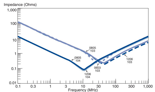
FIGURE 6. Impedance versus Frequency X7R Dielectric
