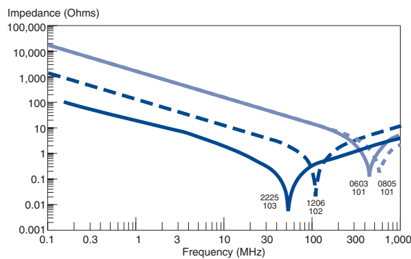
FIGURE 5. Impedance versus Frequency C0G Dielectric
