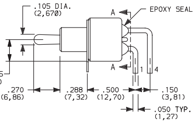
Actuator Shown In Pos. 1 .125 TYP. (3,18) Terminals & Support
