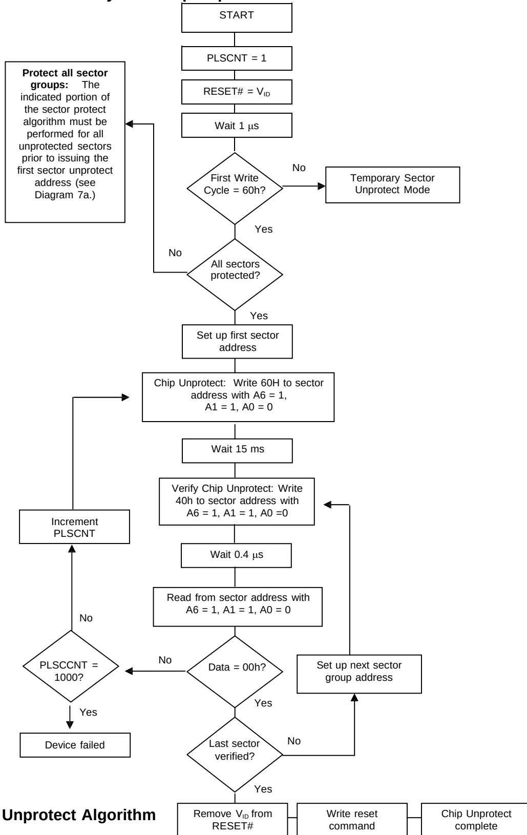
Flowchart 7b. In-System Chip Unprotect Flowchart
