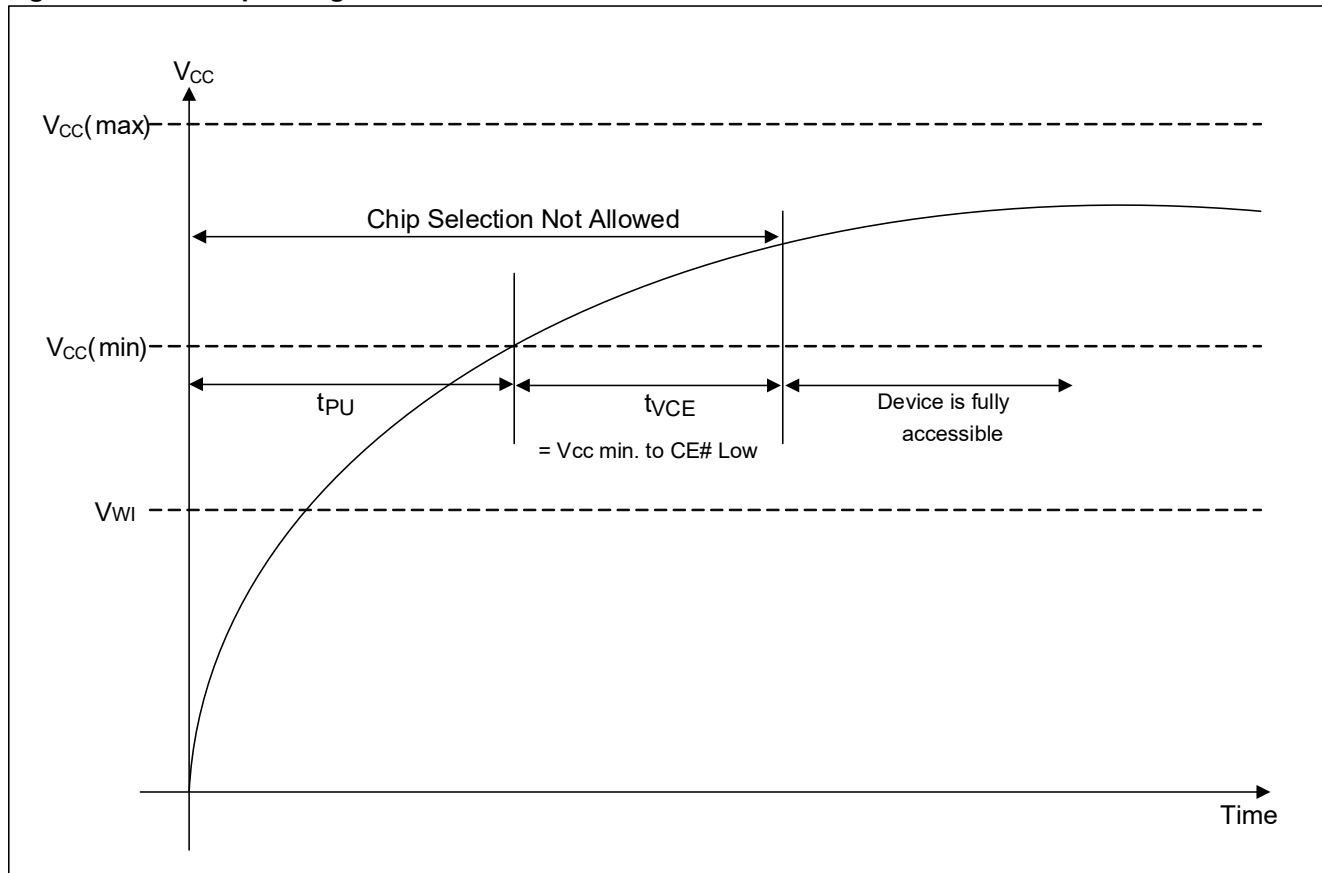
Figure 9.6 Power up timing
