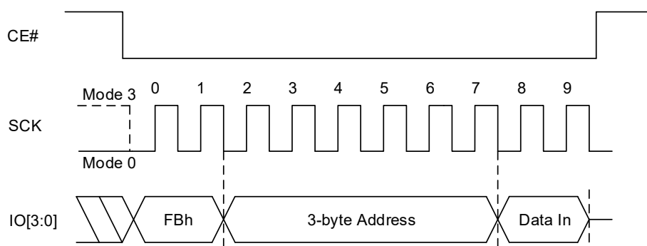
Figure 8.111 Write DYB Sequence In QPI Mode (FBh [EXTADD=0], 3-byte address)
