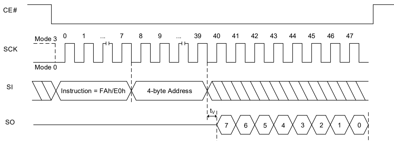
Figure 8.107 Read DYB Sequence In QPI Mode (FAh [EXTADD=0], 3-byte address)
