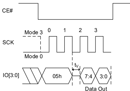
Figure 8.47 Read Status Register Sequence In QPI Mode
