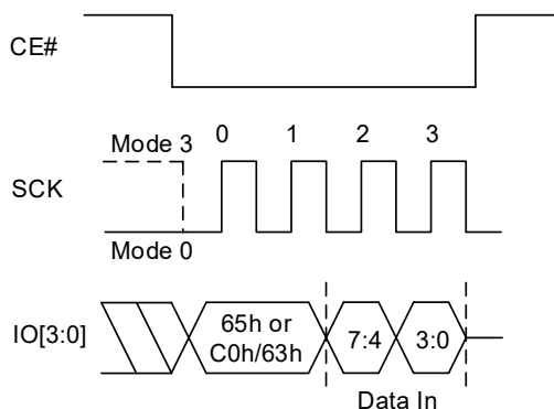
Figure 8.61 Set Read Register Sequence In QPI Mode
