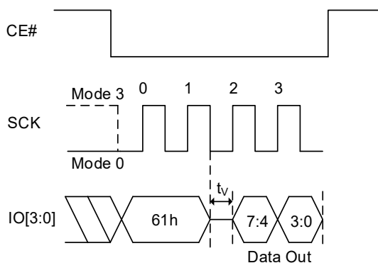
Figure 8.65 Read Read Register Sequence In QPI Mode
