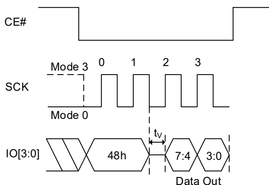
Figure 8.51 Read Function Register QPI Sequence
