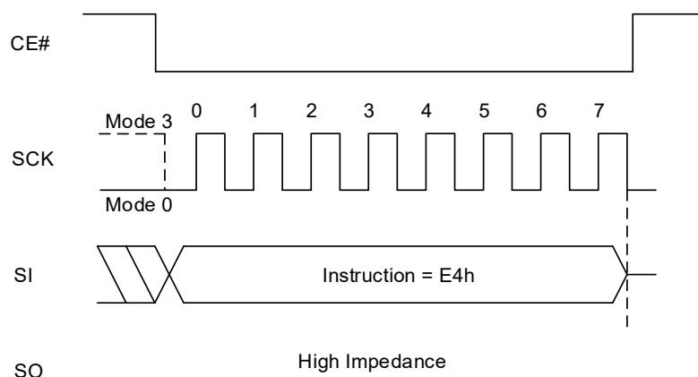
Figure 8.119 Erase PPB Sequence In SPI Mode
