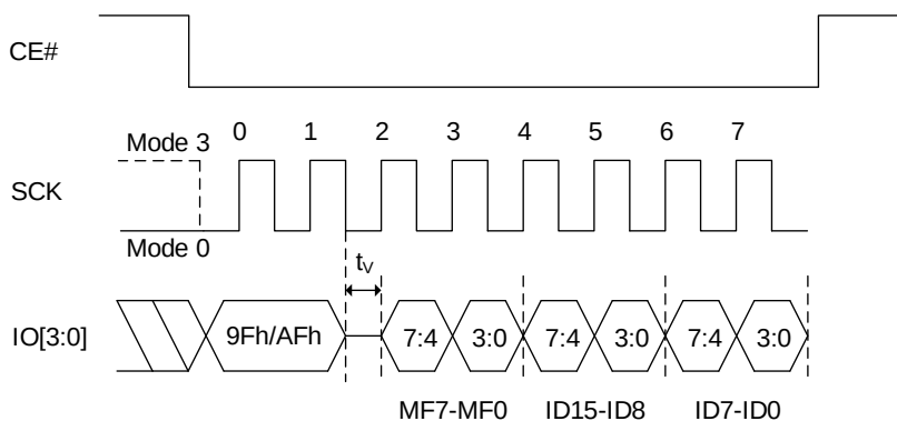
Figure 8.72 RDJID and RDJIDQ (Read JEDEC ID) Sequence In QPI Mode
