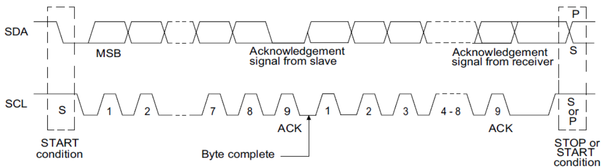
Data Transfer on the I 2 C Bus
